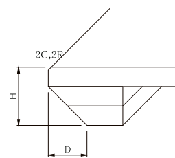
舟型面取
